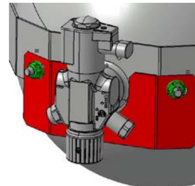
Firewall bracket fastening. The support is also checked in case of vehicle inspection (Italy Market: each 4 years)
