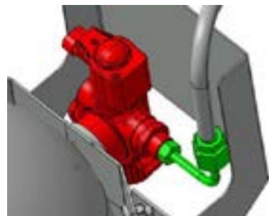
High-pressure hose connection to the check valve on the solenoid valve
