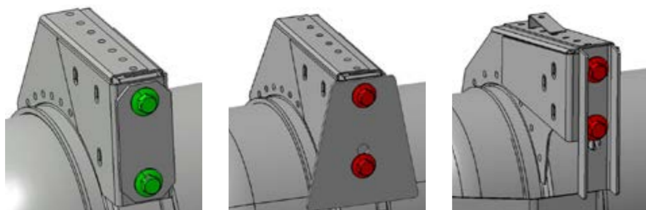
Tank support brackets to chassis and rear cross member fastening with stiffening plates
